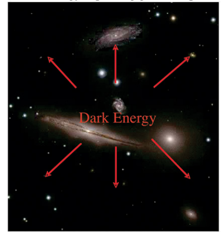
Dark energy is pushing galaxies apart.
